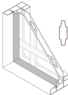
1" Sculptured Internal Grid
