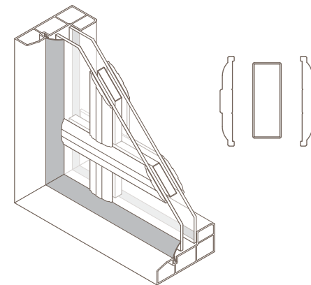
1-1/8" SDL (Simulated Divided Lite) Grid Bar with Internal Shadow Bars
