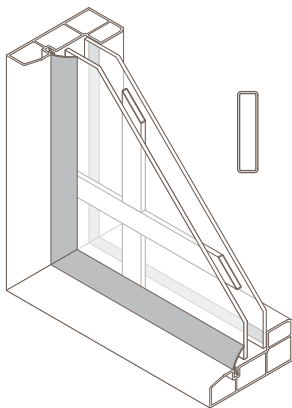
3/4" Flat Internal Grid
